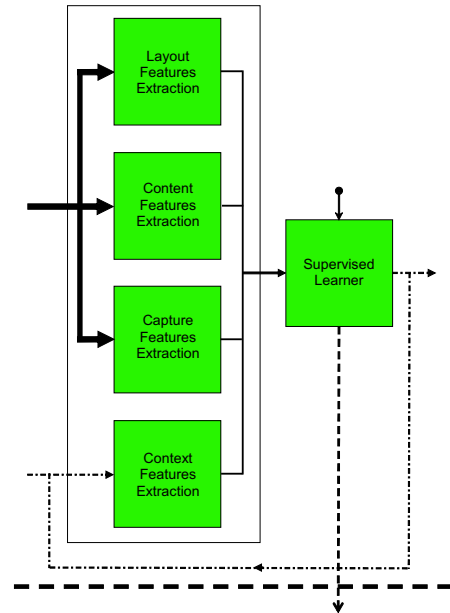
Figure 6: Feature extraction and classification in the style analysis step, special case of Fig. 2.
