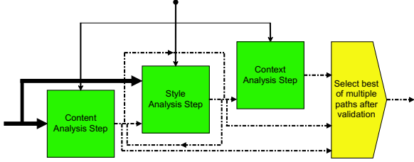
Figure 3: The semantic pathfinder for one concept, using the conventions of Fig. 1.
