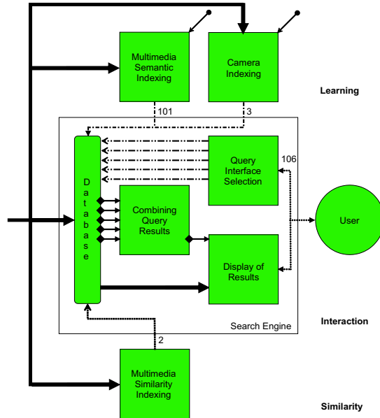
Figure 9: The lexicon-driven paradigm for multimedia retrieval combines learning, similarity, and interaction. It learns to detect a lexicon of 101 semantic concepts together with 3 types of camera work. In addition, it computes 2 similarity distances. A search engine then presents 2 interfaces for query-by-similarity, 3 interfaces for query-by-camera-work, and 101 interfaces for query-by-concept. Based on interaction a user may refine search results until an acceptable standard is reached.
