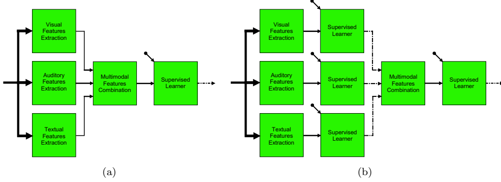
Figure 5: (a) General scheme for early fusion. Output of unimodal analysis is fused before a concept is learned. (b) General scheme for late fusion. Output of unimodal analysis is used to learn separate scores for a concept. After fusion a final score is learned for the concept. We use the conventions of Fig. 1.
